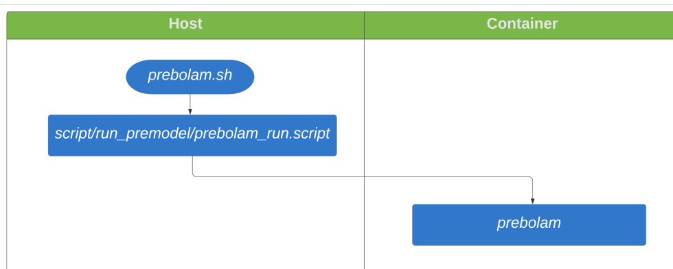
Figure 4: PreBOLAM
