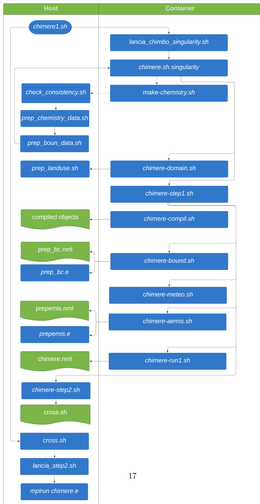
Figure 7: CHIMERE v2014b
