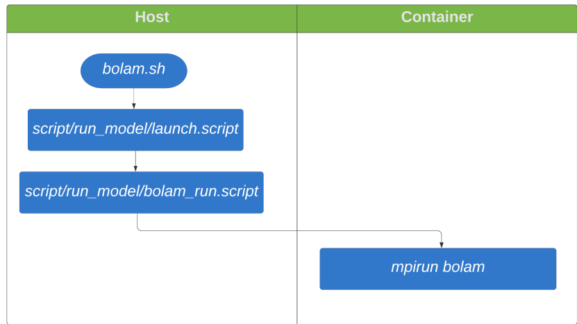
Figure 5: BOLAM
