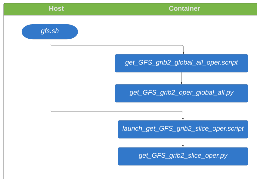
Figure 2: GFS
