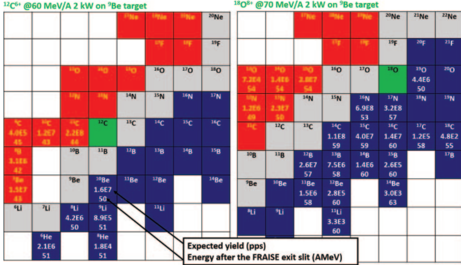
Fig. 2. – Left: simulation of RIBs achievable with FRAISE, using ^{12}\text{C} as the primary beam. Right: simulation of RIBs achievable with FRAISE, using ^{18}\text{O} as the primary beam. See text for details.
