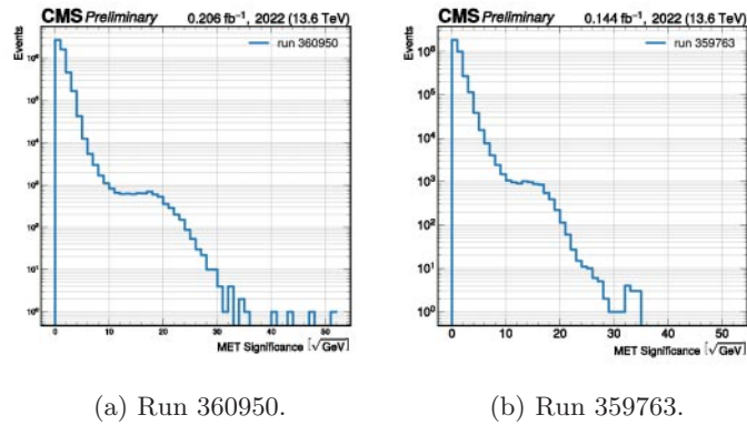
Fig. 3. – Histograms of METSig for the two runs under study, an anomalous shape is evident in both.
