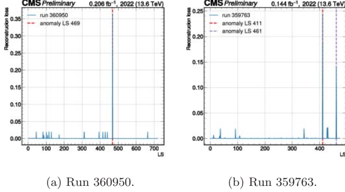
Fig. 4. – Reconstruction loss for the two runs under study showing the presence of a limited set of high peaks.
