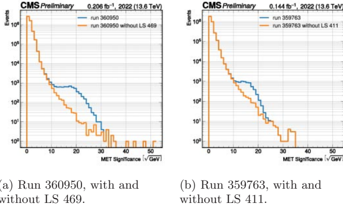
Fig. 5. – The two runs with and without the LSs responsible of the anomaly.
