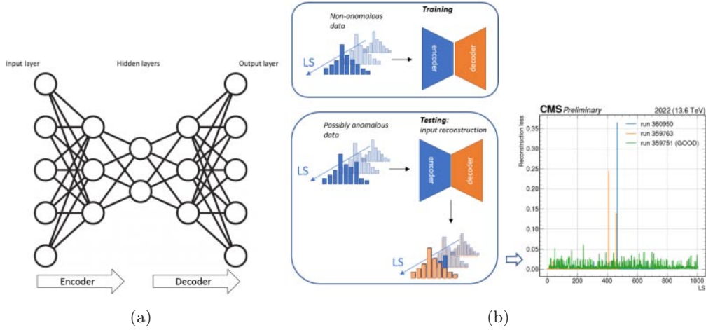
Fig. 2. – Structure of the Under-complete AE (the number of nodes is just indicative) (a) and scheme of training and testing steps for the model (b).
