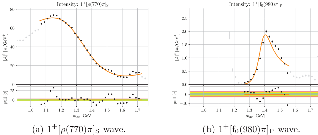
Fig. 1. – Intensities as functions of m_{3\pi} for the partial-wave decompositions (black and grey points), with statistical uncertainties shown, and the prediction of the resonance-model fit (orange lines) to the black points.
