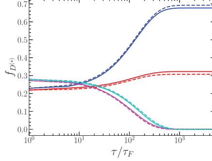
Fig. 1. – Proper-time evolution of the charm-meson fractions f_{D^0} (blue), f_{D^+} (red), f_{D^{*0}} (cyan), and f_{D^{*+}} (magenta). The four fractions add up to 1.
