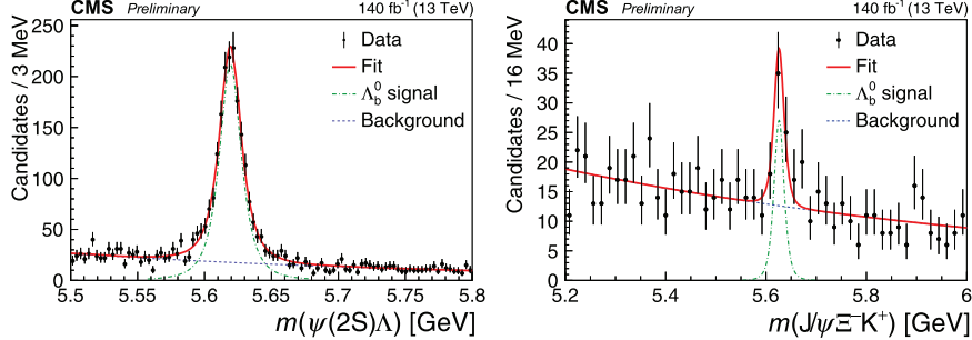
Fig. 3. – The measured \Psi(2S)\Lambda invariant mass distribution with the fit results overlaid (left) [10]. The measured J\Psi\xi^-K^+ invariant mass distribution with the fit results overlaid (right).
