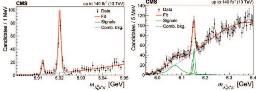
Fig. 1. – Invariant mass distribution of the selected \Lambda_b^0 \pi^+ \pi^- candidates near the kinematic threshold (left) and in the high-mass region (right) [2]. Four signals are considered corresponding to the known \Lambda_b excitations: \Lambda_b(5912) , \Lambda_b(5920) , \Lambda_b(6146) , \Lambda_b(6152) . An additional contribution is introduced to describe the broad enhancement observed in the region below 6.1 GeV.
