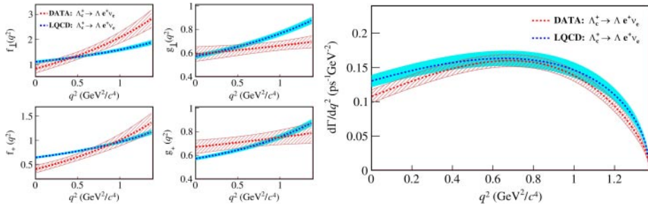
Fig. 1. – The four figures on the left show comparison of form factors with LQCD calculations. The bands show the total uncertainties. The figure on the right shows comparison of the differential decay rates with LQCD predictions. The band shows the total uncertainty.
