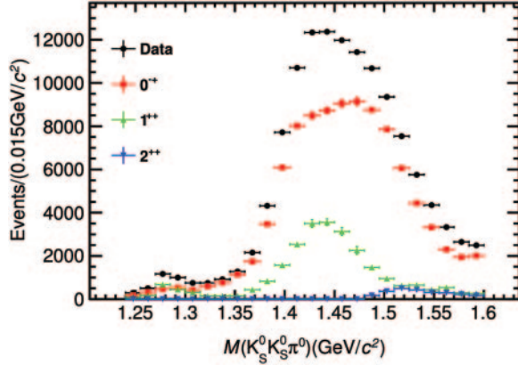
Fig. 2. – K_S^0 K_S^0 \pi^0 intensity spectra for the dominant spin-parity components obtained from MI PWA results. Only statistical uncertainties are reported for data, while the uncertainties on the others are obtained from PWA in each bin.
