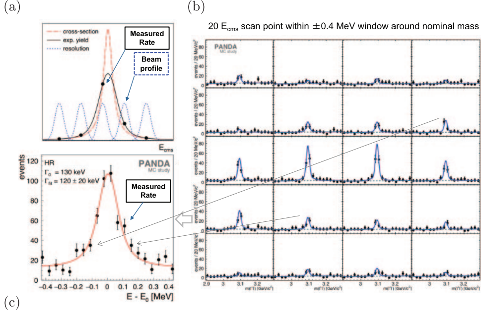
Fig. 2. – Illustration of a MC-simulated scan experiment example ( \sigma_s = 100 nb, Breit-Wigner width \Gamma_0 = 130 keV, two days of data taking per E_{\text{cms}} position, HR mode) [8]. (a) Schematic to explain the resonance energy scan principle. (b) Simulated and reconstructed invariant dilepton spectra at each energy scan position (going from left to right, top to bottom step-wise through the energy range ( E - E_0 )). (c) The resultant energy-dependent event yield distribution around the nominal centre-of-mass energy E_0 = 3.872 GeV is fitted with a function to extract the parameter of interest; in this example an assumed Breit-Wigner width \Gamma_0 .
