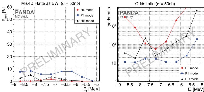
Fig. 5. – Left: sensitivity in terms of the mis-identification probability P_{\text{mis}} to wrongly assign the Breit-Wigner line shape instead of the correct Flatté-like line shape as a function of the Flatté energy parameter E_{\bar{f}} , whereas P_{\text{mis}} = 50\% corresponds to “indistinguishable”. Right: the correspondingly computed so-called “odds”, i.e. , the number of correct assignments per wrong one, defined as \text{odds} := (1 - P_{\text{mis}})/P_{\text{mis}} . Using this measure, the expected performance is at least ten times better than “indistinguishable”.
