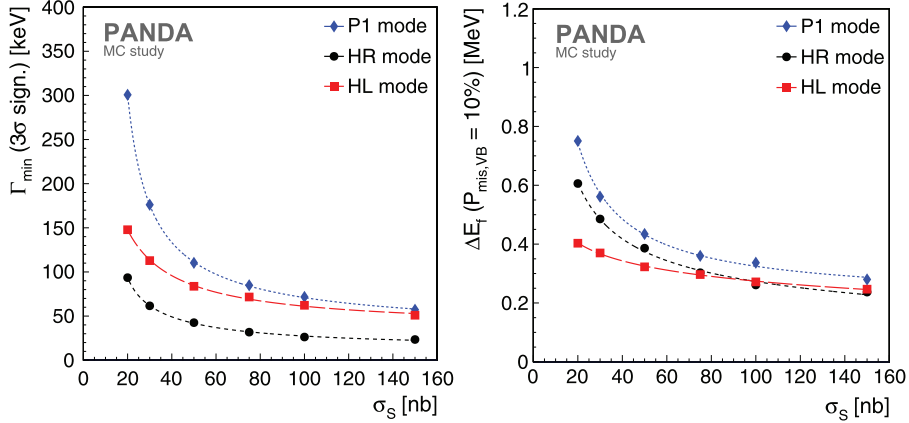
Fig. 3. – Summary of results of the sensitivity study for an absolute (Breit-Wigner) decay width measurement [8]. Left: sensitivity in terms of the minimum decay width \Gamma_{\min} that can be measured with a relative precision of 33% as a function of the assumed input \sigma_S . Right: sensitivity for line-shape measurements via the E_f parameter (molecule case) to distinguish between a bound and a virtual state scenario in terms of the probability to mis-identify a virtual state as a bound state.
