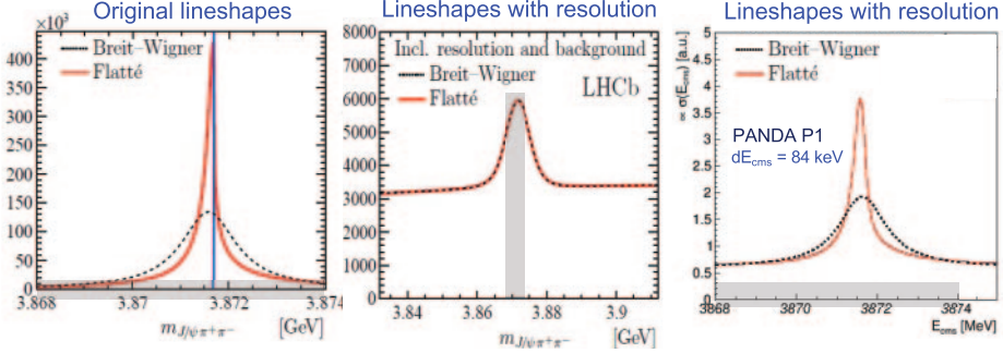
Fig. 4. – Comparison of the Breit-Wigner and Flatté-like line shapes without and with the LHCb and PANDA resolutions convolved. Left: the two line shapes (Breit-Wigner vs. Flatté-like) obtained from the fit to the LHCb data [13]. Centre: the same two line shapes when including backgrounds and resolution, i.e. convolved with the detector resolution. Due to the resolution, the two line shapes cannot be distinguished based on the LHCb data. Right: the same two line shapes (Breit-Wigner vs. Flatté-like) convolved with the PANDA beam energy resolution expected for the initial phase (P1) of the experiment. Thanks to the excellent beam energy resolution, they are well distinguishable with PANDA at HESR.
