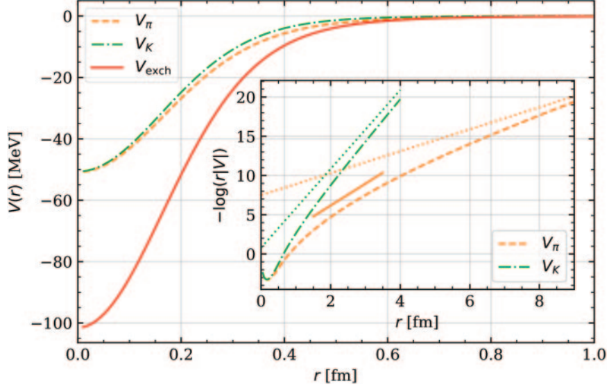
Fig. 1. – The form of the interaction potential in the di- J/\psi system stipulated by the soft-gluon exchanges hadronised at large distances in the form of two-pion and two-kaon exchanges. The inlay zooms the large-separation region and demonstrates the asymptotic behaviour of the different contributions. Adapted from [18].
