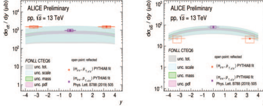
Fig. 2. – (Color online) Preliminary y -differential charm (left) and beauty (right) cross-sections measured in pp collisions at \sqrt{s} = 13 TeV. The red markers represent the new ALICE measurement at forward rapidity, obtained with measuring dimuons in 4 < m_{\mu\mu} < 9 GeV/ c^2 , while the midrapidity result was obtained with the dielectron measurement [8] (purple markers). Results are compared to FONLL calculations [6].
