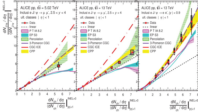
Fig. 4. – (Color online) Self-normalized yield as a function of the self-normalized charged-particle multiplicity measured at midrapidity for forward rapidity J/\psi in pp collisions at \sqrt{s} = 5.02 TeV (left panel) and at \sqrt{s} = 13 TeV (middle panel), and for midrapidity J/\psi at \sqrt{s} = 13 TeV (right panel).
