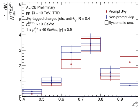
Fig. 3. – (Color online) New preliminary measurement of prompt and non-prompt J/\psi production as a function of z_{J/\psi}^{\text{ch}} ( i.e. , the fraction of the jet momentum carried by the J/\psi ) in charged jets for pp collisions at \sqrt{s} = 13 TeV at midrapidity.
