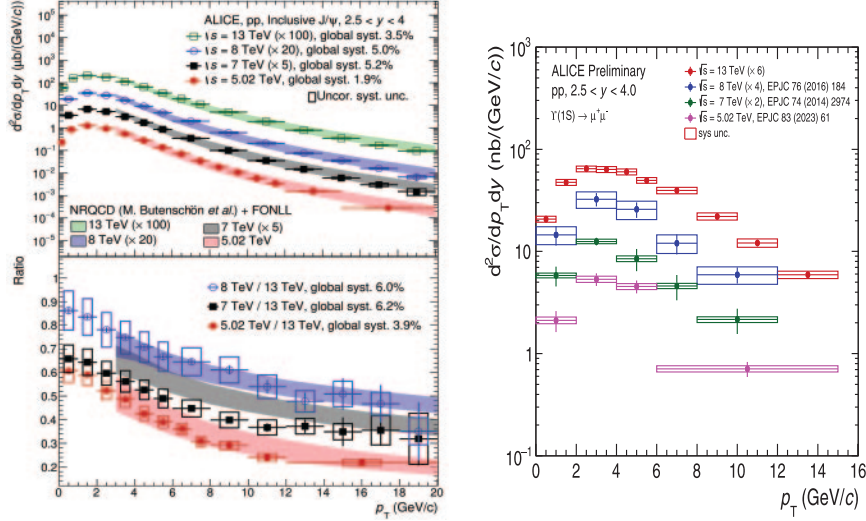
Fig. 1. – (Color online) Inclusive p_T -differential quarkonium cross-sections (left panel for J/\psi , right panel for \Upsilon(1S) ), measured in pp collisions at \sqrt{s} = 5.02, 7, 8 and 13 TeV. The J/\psi results have been compared with NRQCD [4] calculations, coupled with FONLL [6] to include the non-prompt J/\psi contribution from b -hadron decays.
