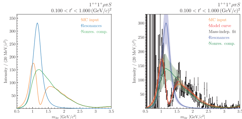
Fig. 2. – Left: intensity of input model (orange) split in resonant (blue) and non-resonant (green) components. Right: comparison of the two different fitting methods. The binned fit (black points) shows large statistical uncertainties. The new method (red) recovers the input model (orange) with high accuracy. It also correctly separates the components (blue and green). More examples can be found in [1].
