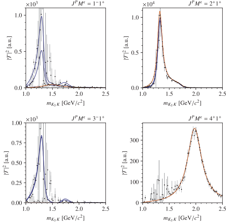
Fig. 1. – Partial-wave intensities of the ambiguous amplitudes. The model and calculated solutions are drawn as orange and blue curves, respectively. The intensities obtained in the PWA fit are shown as black dots with grey error bars. See also [1].
