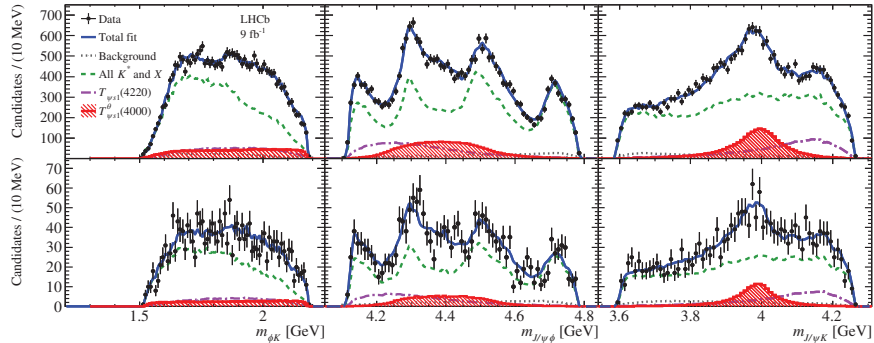
Fig. 2. – (Color online) The (left) \phi K , (middle) J/\psi \phi and (right) J/\psi K mass distributions, overlaid with projections of a simultaneous amplitude fit of the (upper) B^+ \rightarrow J/\psi \phi K^+ and (lower) B^0 \rightarrow J/\psi \phi K_S^0 samples collected by the LHCb experiment. A GPU-based fit framework is used for the amplitude analysis. The red area shows the contribution of the (upper) T_{\psi s 1}^{\theta}(4000)^+ and (lower) T_{\psi s 1}^{\theta}(4000)^0 tetraquark candidates [11].
