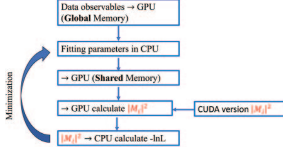
Fig. 1. – The data flow between the GPUs and CPUs in the fit framework of the B^0 \rightarrow J/\psi K_S^0 \phi amplitude analysis [11]. Data observables saved in the GPU global memory include all amplitude terms that keeps invariant during the minimization procedure.
