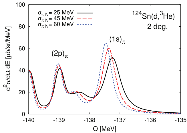
Fig. 1. – Formation cross sections of the deeply bound pionic atoms in ^{123}\text{Sn} by the (d, {}^3\text{He}) reaction for three different values of \sigma calculated in ref. [6]. The scattering angle of the emitted {}^3\text{He} nucleus is fixed to be 2^\circ in the laboratory frame. The experimental energy resolution is assumed to be 150 keV.
