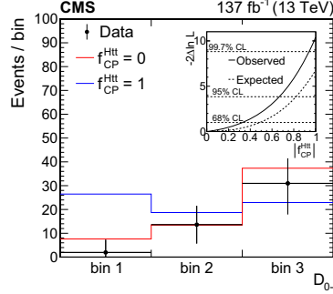
Fig. 1. – The distribution of events weighted by S/(S + B) ( S = Signal, B = Background) in three bins of the D_{0-} discriminant. In this display, leptonic/hadronic channels and BDT-bkg categories are combined in the mass range 115 < m_{\gamma\gamma} < 135 GeV and the background contribution, as determined in the fit to data, is subtracted. The inner panel shows the likelihood scan for |f_{CP}^{Htt}| [4].
