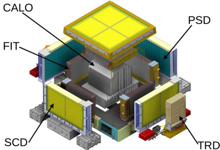
Fig. 3. – Schematic picture of the HERD detector: at the center the calorimeter (CALO), going outside the Fiber Tracker (FIT), on the outermost the Plastic Scintillator Detector (PSD) and the Silicon Charge Detector (SCD). On one side we also have the Transition Radiation Detector (TRD).
