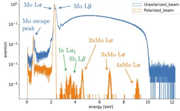
Fig. 2. – Spectra of unpolarized and polarized beams produced by the MXR tube. The polarized spectrum shows different diffraction orders and the crystal fluorescence (In L_\alpha and Sb L_\beta ).
