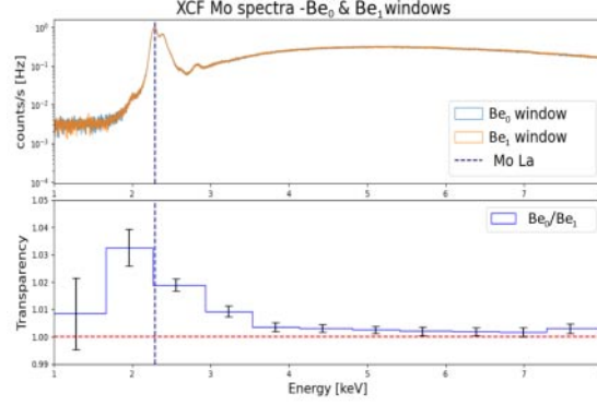
Fig. 5. – Relative transparency of the two windows.
