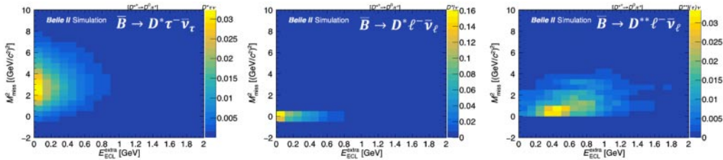
Fig. 1. – E_{\text{ECL}} vs. M_{\text{miss}}^2 distribution of three different samples. \bar{B} \rightarrow D^* \tau^- \nu is on the left plot, \bar{B} \rightarrow D^* \ell^- \nu is in the center, and \bar{B} \rightarrow D^{**} \ell^- \nu is in the right plot.
