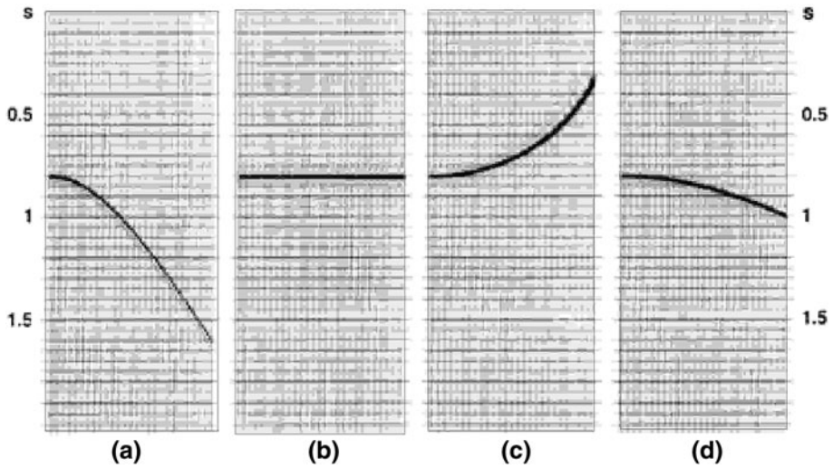
Fig. 5 Variations of the hyperbola of a seismic reflector according with the velocity values used in the NMO correction
