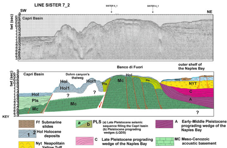
Fig. 12 Regional seismic profile Sister7_2 and corresponding geological interpretation. MC Acoustic basement. Meso-Cenozoic carbonates cropping out offshore the Sorrento Peninsula and the Capri island. A Early Pleistocene relic prograding wedge, representing the lower unit in the stratigraphic architecture of the Naples Bay, characterized by oblique prograding clinoforms and parallel reflectors (perpendicular to the direction of progradation). B Late Pleistocene prograding wedge representing the upper unit in the stratigraphic architecture of the Naples Bay, characterized by low-angle sigmoidal to oblique clinoforms and parallel reflectors (perpendicular to the direction of progradation), supplied by the palaeo-Sarno river mouth. Pls Late Pleistocene seismic sequence representing the basin filling of the Capri Basin. Hol Holocene deposits, characterized by parallel and continuous seismic reflectors in the Capri Basin. Hol Holocene deposits on the outer shelf of the Naples Bay characterized by alternances of marine and volcanoclastic sediments; interlayered slide deposits ( Bb ). Holb Holocene deposits, characterized by an acoustically transparent seismic facies in correspondence to channel–levee complexes in the Dohrn canyon's thalweg
